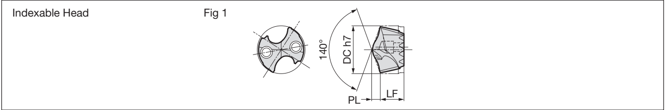
Indexable Head MEL Type Diameter \varnothing 12.0 to 17.3mm Dimensions (mm)
