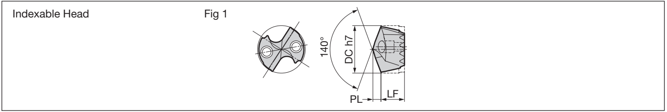
Indexable Head MSL Type Diameter ø22.8 to 28.1mm Dimensions (mm)
