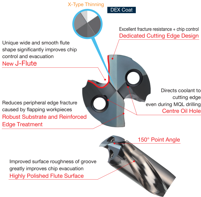
MB Type for Bridge Good chip control
